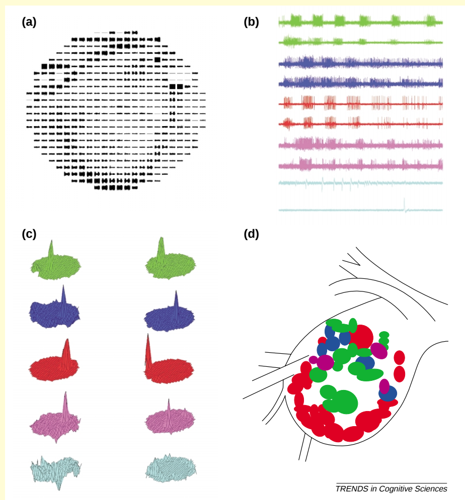
Fig. 2. (a) Mean 448-pixel image from array of 448 photodiode-detector array over 8 seconds (sampling rate 1kHz). (b) Temporal independent components (tICs) were classified into five colour-coded classes. Each tIC class identifies a set of neurons with similar firing patterns. One tIC class (light blue, at bottom) identifies signal artifacts. (c) The relative contribution of each detector to each colour-coded tIC, as denoted by height. Only tICs corresponding to single neurons defined spatially localized clusters. By contrast, tICs associated with signal artifacts defined spatially distributed detectors (bottom). (d) Spatial positions of neurons associated with each colour-coded tIC class. (Reproduced, with permission, from Ref. c.)
